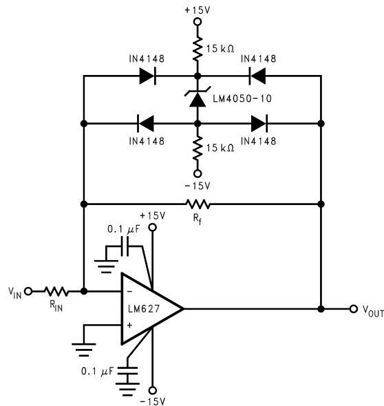
Figure 12. Bounded Amplifier
