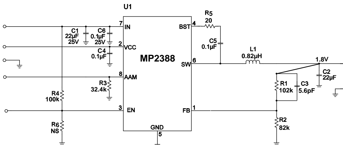
Figure 13: V_{IN} = 12V , V_o = 1.8V , I_o = 1A
