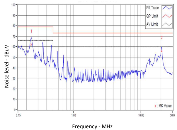
Figure 12. Conducted Emissions
