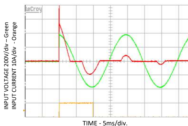
Figure 4. Inrush performance
