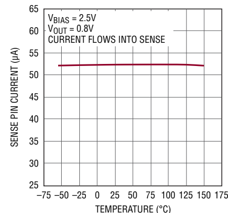
SENSE Pin Current
