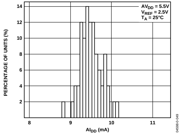
Figure 15. A_{lDD} Histogram
