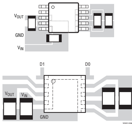
Figure 6. Recommended Layouts
