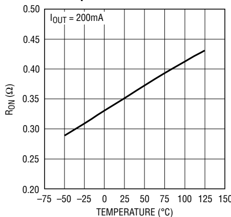
R_{\text{ON}} from V_{\text{BUS}} to V_{\text{OUT}} vs Temperature
