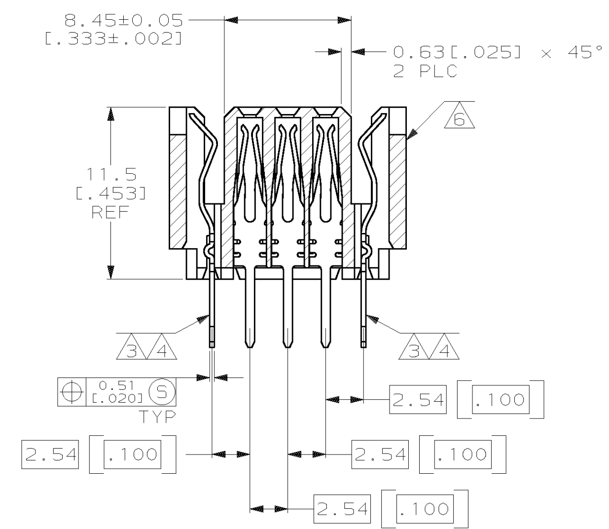
SECTION X-X
