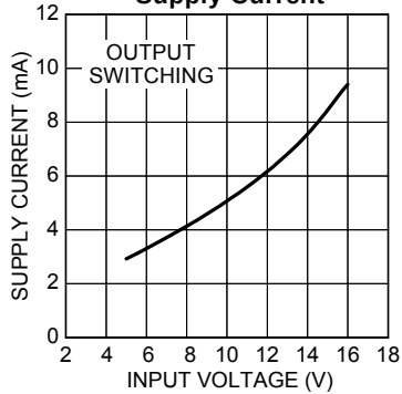
PWM-Mode Supply Current
