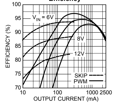
5V Output Efficiency
