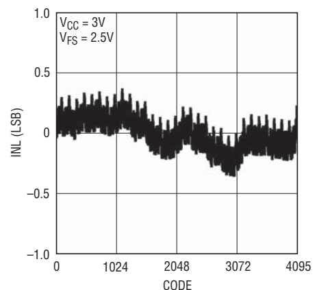
Integral Nonlinearity (LTC2640A-LZ12)
