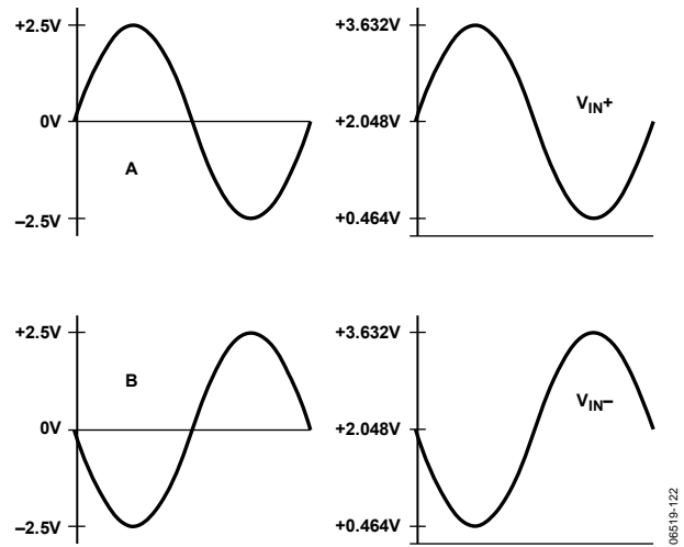
Figure 31. Differential Amplifier Signal Conditioning
