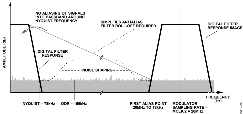
Figure 28. Antialias Example Using the AD7765 in Normal Mode, Decimate 128x Using MCLK/2 = ICLK = 20\text{ MHz}
