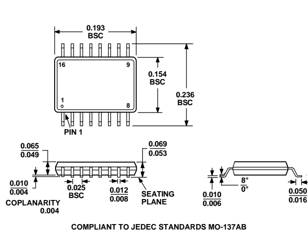
Figure 30. 16-Lead Shrink Small Outline Package [QSOP] (RQ-16)
