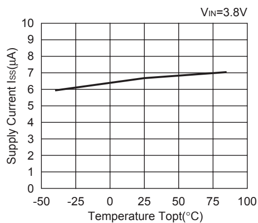
R1163x281x ECO=L
