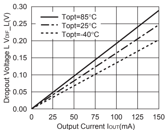
R1163x401x ECO=L
