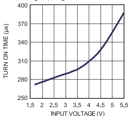
Turn_on Time vs. Input Voltage
