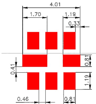
PCB Footprint
