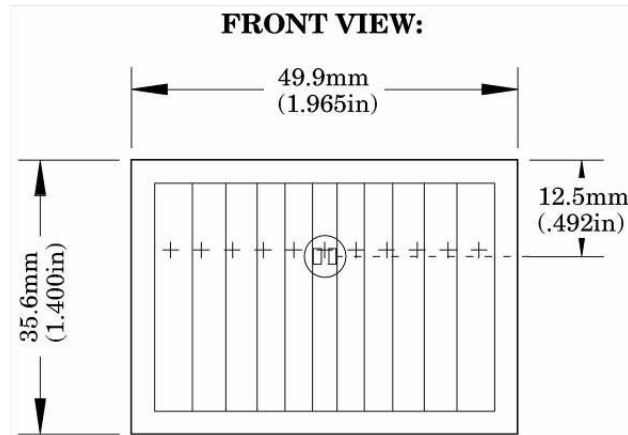
Figure 9. Flat Lens: AA 0.9 GI T1
