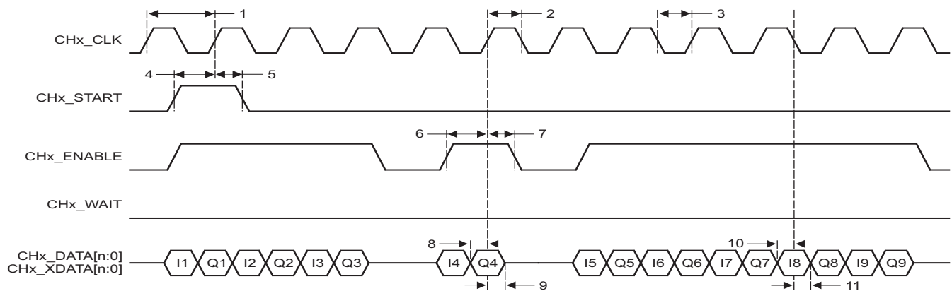
Figure 7-55 uPP Double Data Rate (DDR) Receive Timing
