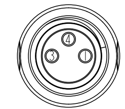
3P C2 Pin Assignments Front View
