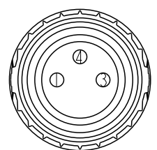
3P C1 Pin Assignments Front View
