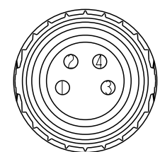
4P C1 Pin Assignments Front View
