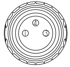
3P CI Pin Assignments Front View
