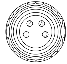
4P CI Pin Assignments Front View
