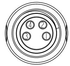
4P C2 Pin Assignments Front View
