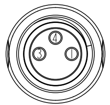
3P C2 Pin Assignments Front View
