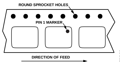
Figure 19. ADM6305/ADM6306 Reel Orientation
