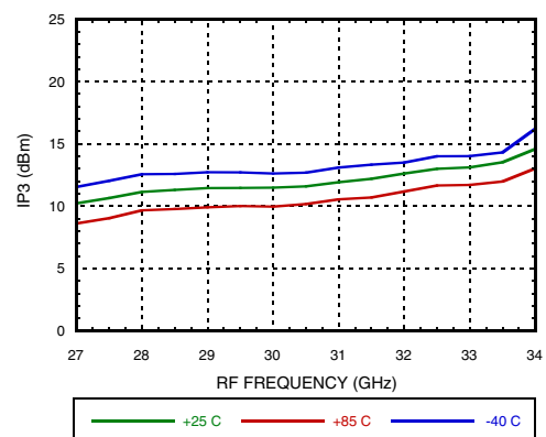
Output IP3 vs. Temperature, USB
