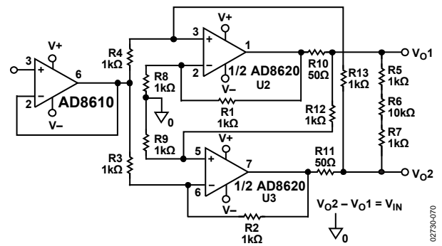
Figure 70. Differential Driver
