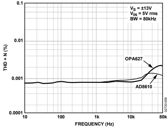
Figure 58. AD8610 vs. OPA627 THD + Noise @ V_{CM} = 0\text{ V}
