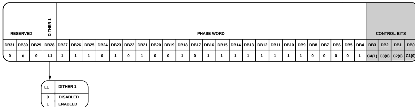
Figure 32. Register 8 (R8)
