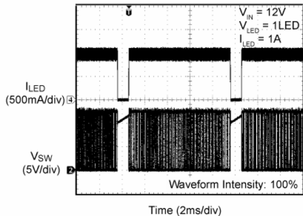
PWM Dimming @ 100Hz (90% Duty Cycle)
