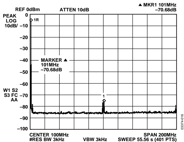
Figure 5. f_{OUT} = 1\text{ MHz} , f_{CLK} = 400\text{ MSPS} , WBSFDR
