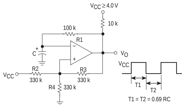
Figure 8. Squarewave Oscillator
