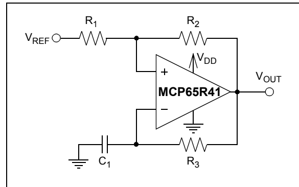
FIGURE 4-11: Bistable Multi-Vibrator.
