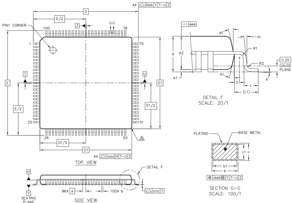
Figure 4.2. LQFP100
