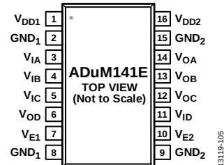
Figure 9. ADuM141E Pin Configuration
