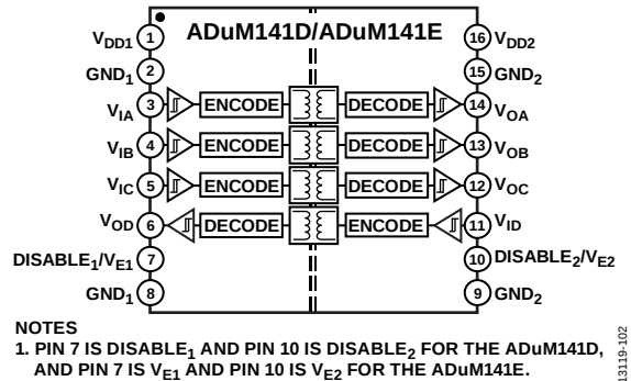
Figure 2. ADuM141D/ADuM141E Functional Block Diagram
