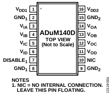
Figure 6. ADuM140D Pin Configuration
