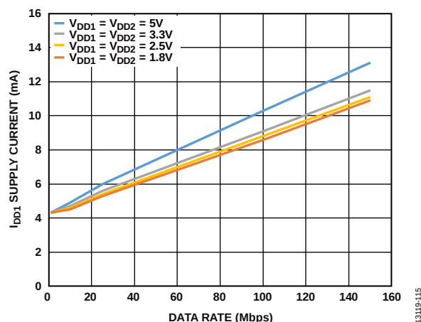
Figure 16. ADuM142D/ADuM142E I_{DD1} Supply Current vs. Data Rate at Various Voltages
