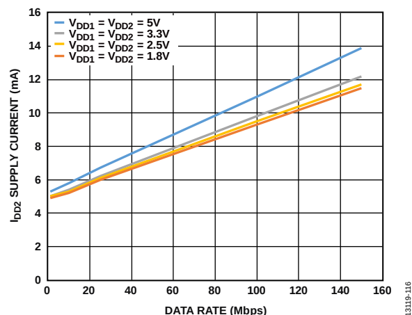
Figure 17. ADuM142D/ADuM142E I_{DD2} Supply Current vs. Data Rate at Various Voltages
