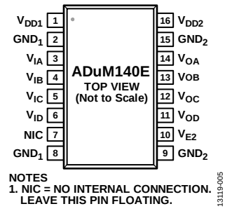
Figure 7. ADuM140E Pin Configuration
