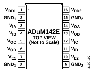
Figure 11. ADuM142E Pin Configuration
