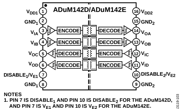
Figure 3. ADuM142D/ADuM142E Functional Block Diagram
