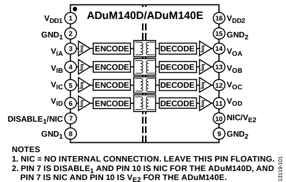
Figure 1. ADuM140D/ADuM140E Functional Block Diagram
