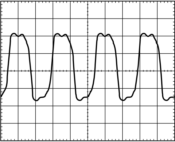
Figure 18. LVPECL Differential Output @ 800 MHz
