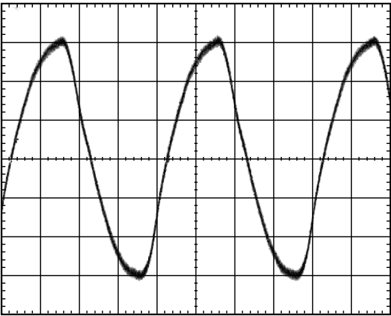
Figure 20. CMOS Single-Ended Output @ 250 MHz with 10 pF Load
