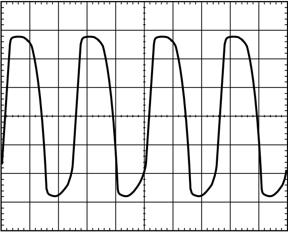
Figure 19. LVDS Differential Output @ 800 MHz
