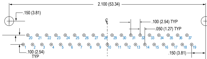
37 SOCKET MWDM-37SBR
