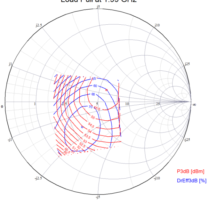
Load Pull at 1.99 GHz
