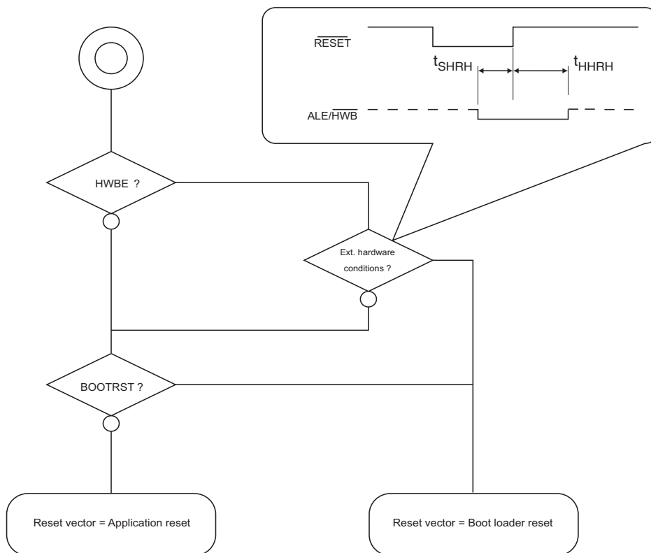
Figure 29-3. Boot process description.
