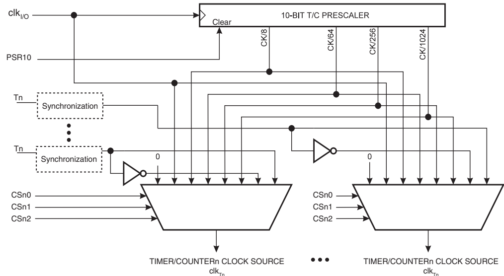
clk_100Mhz 100 MHz 10-BIT T/C PRESCALER
