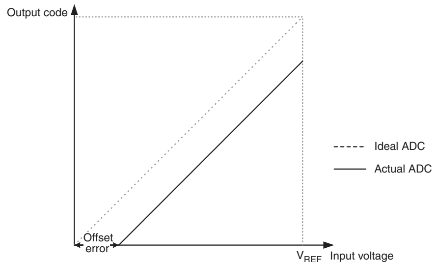
Figure 26-10. Offset error.
