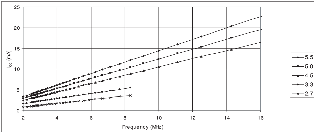
Figure 32-12. Active supply current vs. frequency, T = 25^{\circ}\text{C} .
