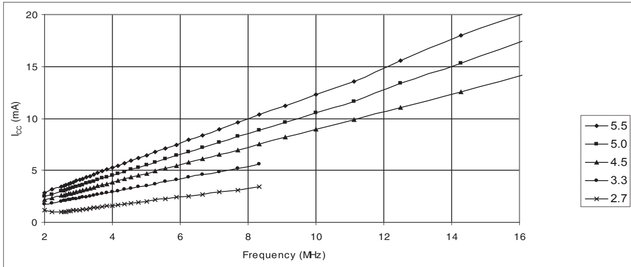
Figure 32-11. Idle supply current vs. frequency, T = 25^{\circ}\text{C} .
