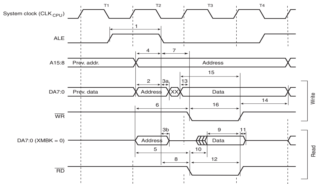
Figure 31-7. External memory timing (SRWn1 = 0, SRWn0 = 0).
