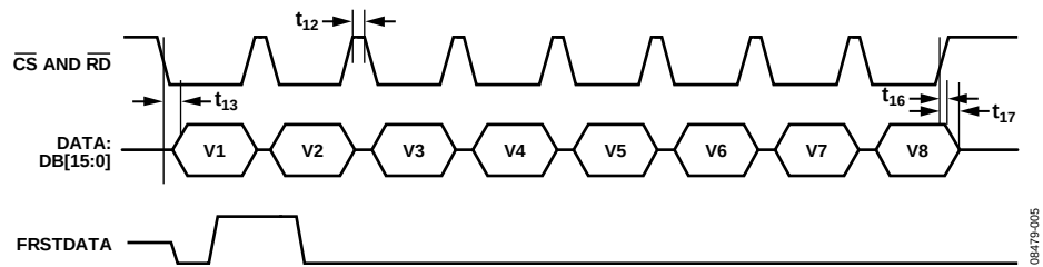
Figure 5. \overline{CS} and \overline{RD} , Linked Parallel Mode
