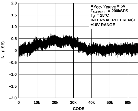
Figure 14. AD7606 Typical INL, ±10 V Range
