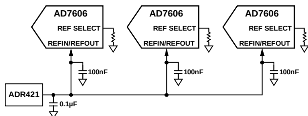
Figure 41. Single External Reference Driving Multiple AD7606/AD7606-6/AD7606-4 REFIN Pins
