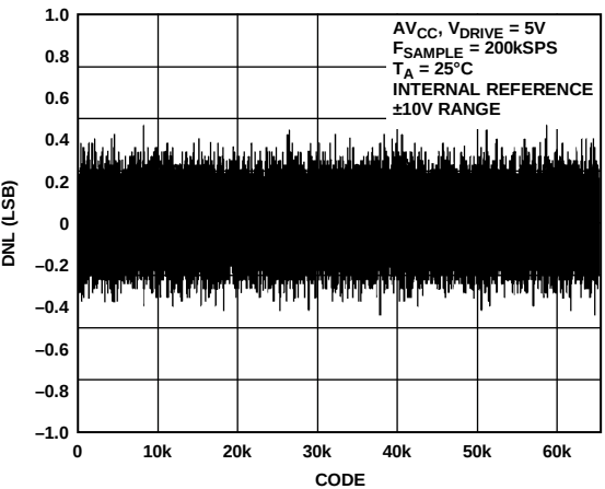
Figure 15. AD7606 Typical DNL, ±10 V Range
