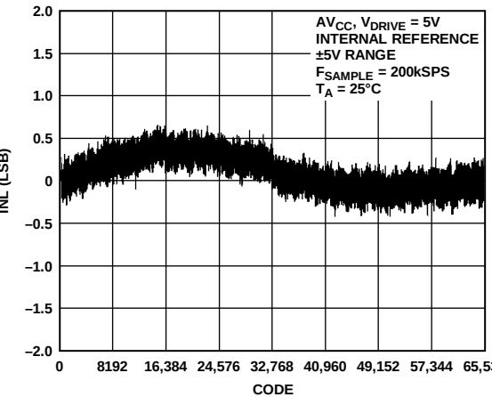
Figure 16. AD7606 Typical INL, ±5 V Range
