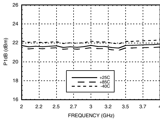
P1dB vs. Temperature [1]
