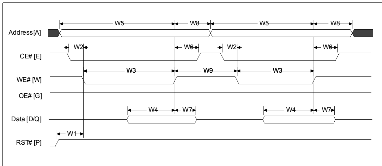
Figure 25: Write-to-Write Timing
