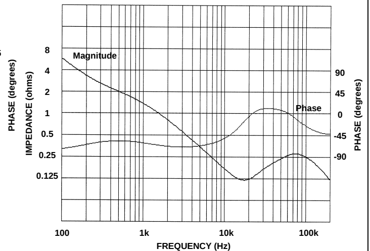
Model N6762A, CC Mode, @50V, 2A
