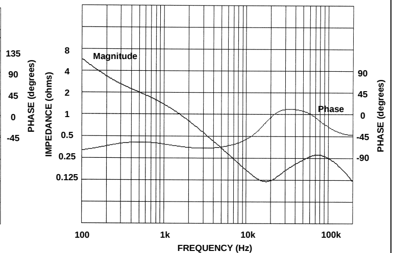
Model N6762A, CC Mode, @50V, 2A
