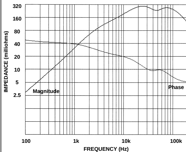
Model N6762A, CV Mode, @50V, 2A
