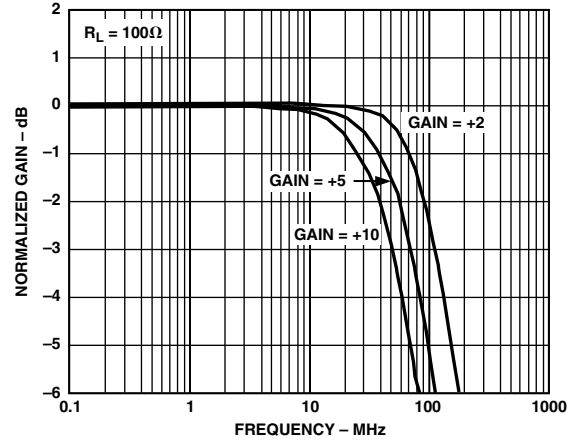
TPC 20. Frequency Response; V_S = \pm 2.5\text{ V}
