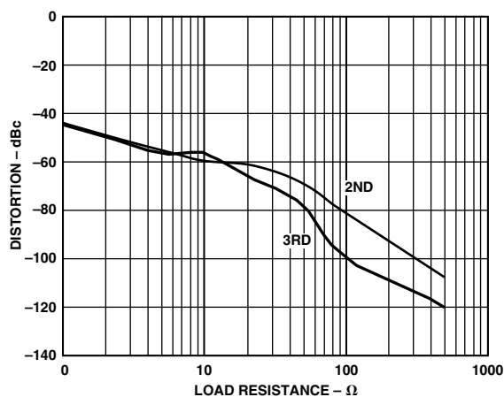
TPC 14. Distortion vs. R_L , V_S = \pm 2.5V , G = +2 , V_{OUT} = 2\text{ V p-p} , f = 1\text{ MHz}
