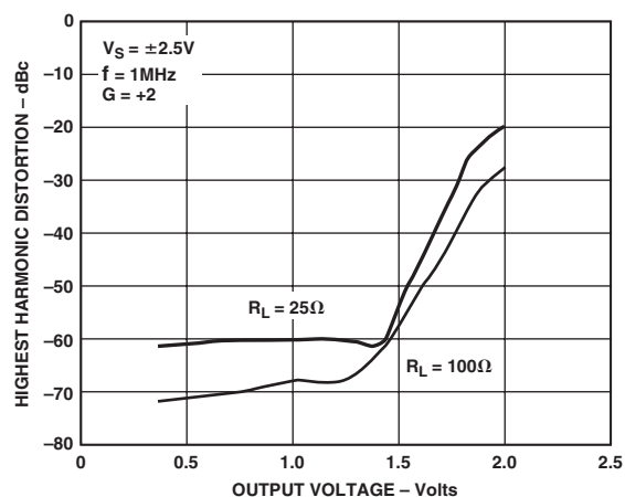
TPC 15. Distortion vs. Output Voltage, V_S = \pm 2.5V , G = +2 , f = 1\text{ MHz}
