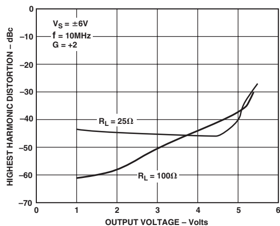
TPC 13. Distortion vs. Output Voltage, V_S = \pm 6V , G = +2 , f = 10\text{ MHz}
