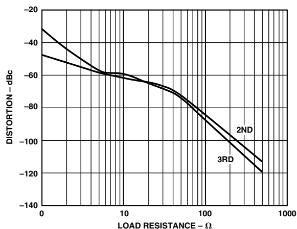
TPC 11. Distortion vs. R_L , V_S = \pm 6V , G = +2 , V_{OUT} = 2\text{ V p-p} , f = 1\text{ MHz}
