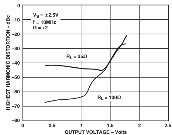
TPC 16. Distortion vs. Output Voltage, V_S = \pm 2.5V , G = +2 , f = 10\text{ MHz}
