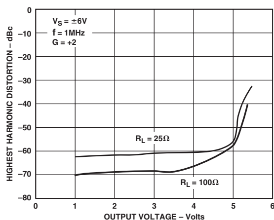
TPC 12. Distortion vs. Output Voltage, V_S = \pm 6V , G = +2 , f = 1\text{ MHz}
