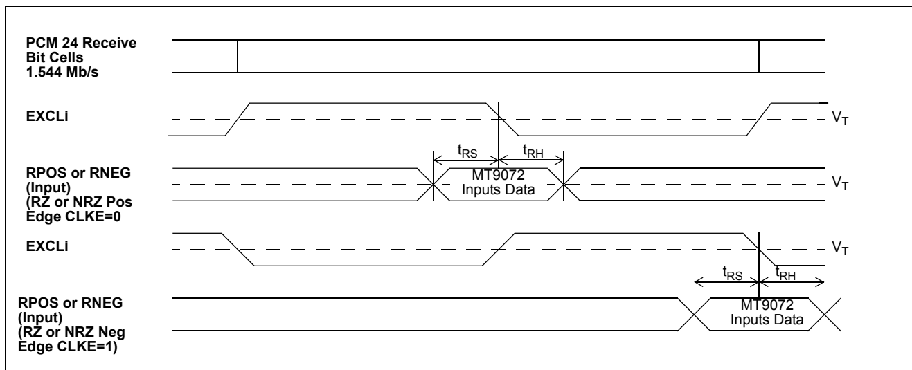
Figure 54 - PCM24 Receive Timing
