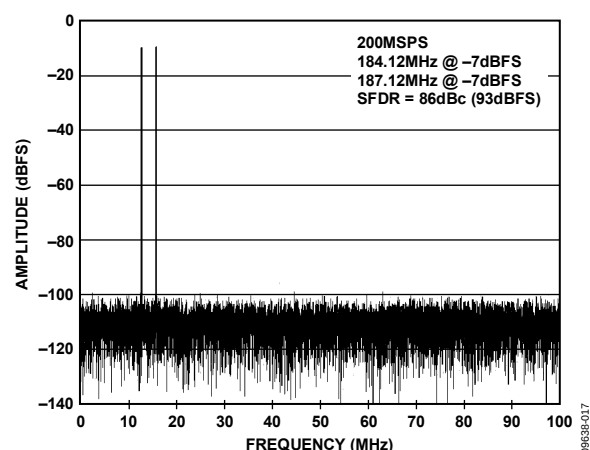
Figure 17. AD6643-200 Two Tone FFT with f_{IN1} = 184.12 MHz, f_{IN2} = 187.12 MHz
