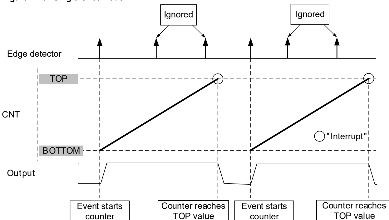
Figure 21-8. Single-Shot Mode
