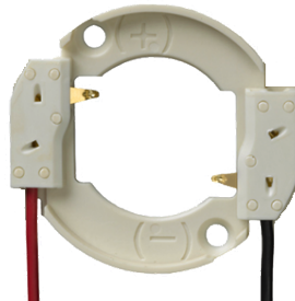
LED Array Holder for Sharp Mega Zenigata (180330-0002)
