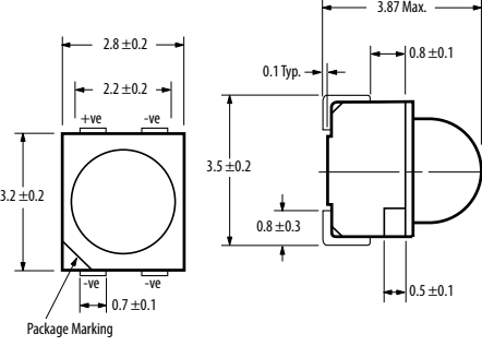
Power PLCC-4 with Lens
