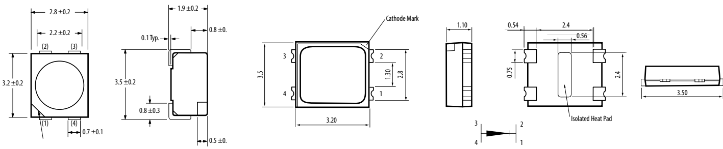
Super 0.5W Power PLCC-4
