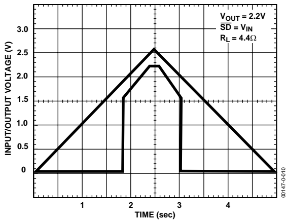
Figure 12. Power-Up/Power-Down
