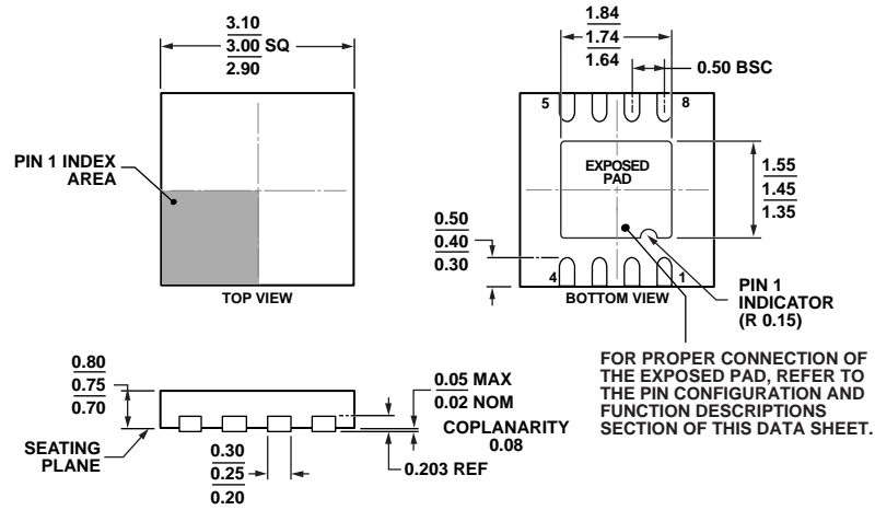
Figure 26. 8-Lead Lead Frame Chip Scale Package [LFCSLP_WD] 3 mm × 3 mm Body, Very Very Thin, Dual Lead (CP-8-13) Dimensions shown in millimeters
